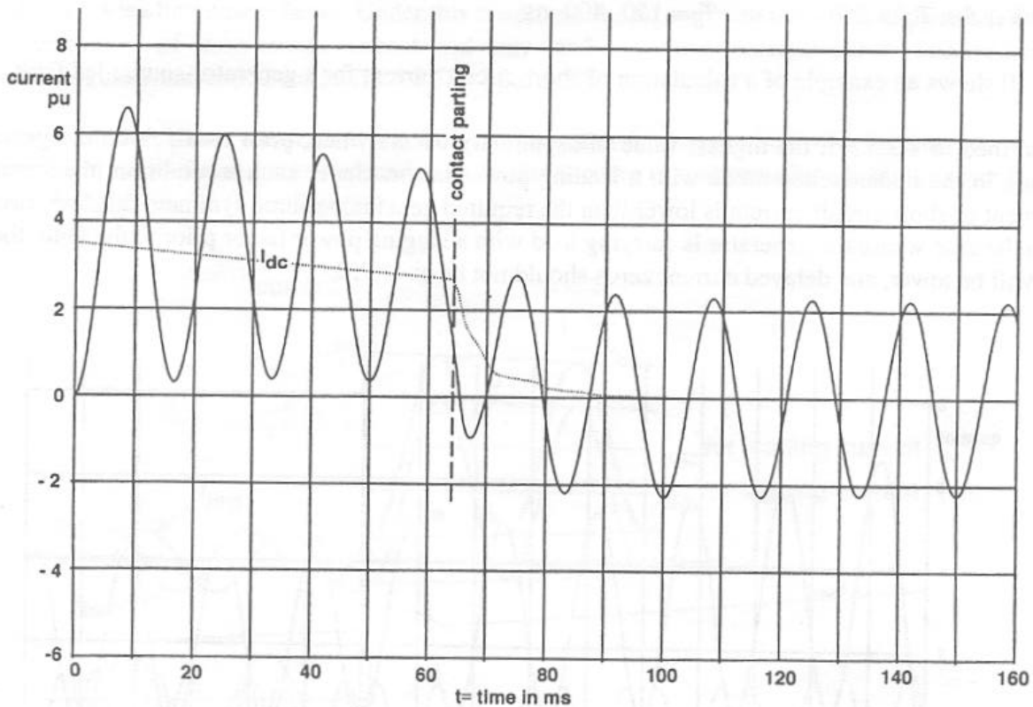
FIGURE 2. Short-circuit Current with Delayed Current Zeroes [1]
