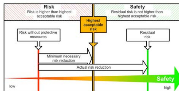
Fig. 1-1 Principles of safety philosophy for low-voltage installations and low-voltage equipment from a technical risk perspective. Reduction of the residual risk through additional measures that lead to clearly falling below the highest acceptable risk ("limiting risk") towards increased safety.
