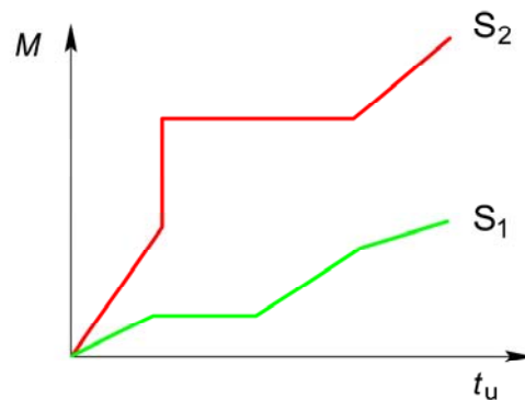
Fig. 2-1 Possible shapes of Damage Interruption Functions ( S_1, S_2 ); M ... damage (or consequential damages) in monetary units 4 , t_u ... duration of interruption of power supply, e. g. in hours
